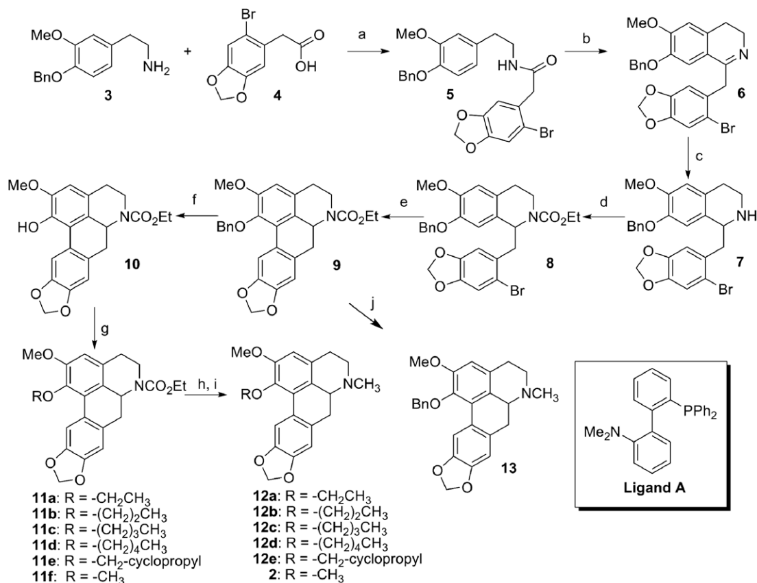
Scheme 1. Reagents and conditions: (a) CDI, THF, rt, 20 h, 90%; (b) \text{PCl}_5 , DCM, 0^\circ\text{C} –rt, 96%; (c) \text{NaBH}_4 , MeOH, 0^\circ\text{C} , 4 h, 99%; (d) ethyl chloroformate, \text{K}_2\text{CO}_3 , DCM, rt, 12 h, 76%; (e) \text{Pd}(\text{OAc})_2 , ligand A, \text{K}_2\text{CO}_3 , (\text{CH}_3)_3\text{CCOOH} , DMA, 130^\circ\text{C} , 17 h, 76%; (f) \text{H}_2/\text{Pd}-\text{C} , MeOH–THF, rt, 38 h, 75%; (g) alkyl bromide, \text{K}_2\text{CO}_3 , acetone, reflux 12 h; (h) \text{LiAlH}_4 , THF, 0^\circ\text{C} , 5 h, 91%; (i) aq HCHO, \text{NaBH}(\text{OAc})_3 , DCM, rt, 24 h, 96%; (j) \text{LiAlH}_4 , \text{Et}_2\text{O} , 0^\circ\text{C} , 5 h, 91%.
